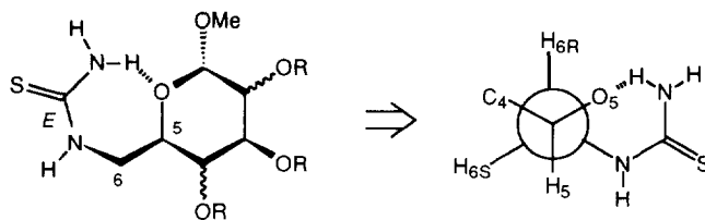
Figure 1. Intramolecular hydrogen bonding in the E rotamer of methyl 6-deoxy-6-thioureido hexopyranosides showing the gauche-trans (gt) disposition at the C 5 –C 6 linkage.
